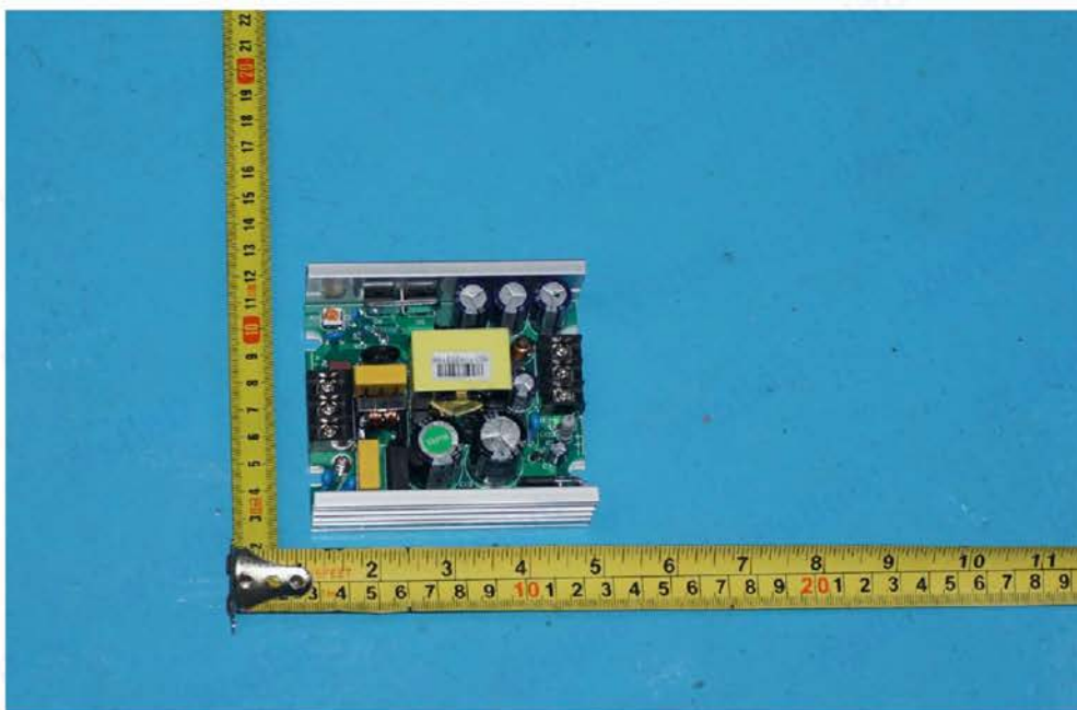
Photo 5: PCB view
